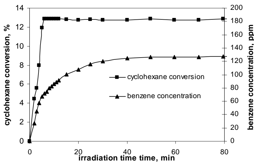
Figure 2 Cyclohexane and benzene outlet concentration as a function of irradiation time (10MoDTA catalyst)
